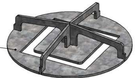
Steel Pottery Expansion Disk n°6
