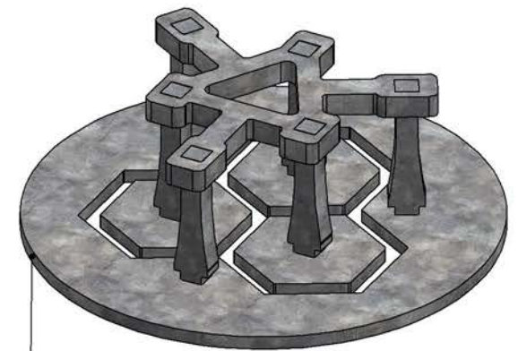
Steel Pottery Extruder Disk n° 111
