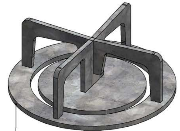
Steel Pottery Extruder Disk n° 1
