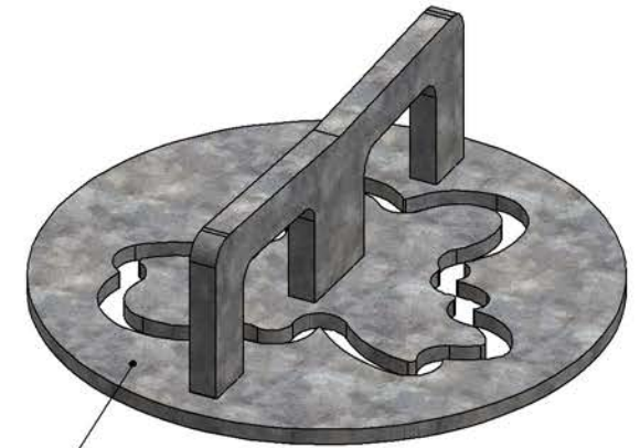
Steel Pottery Extruder Disk n° 23
