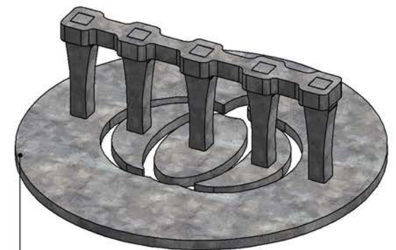
Steel Pottery Extruder Disk n° 109
