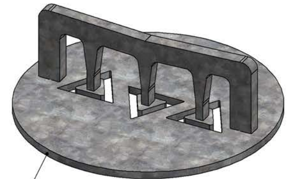
Steel Pottery Extruder Disk n° 10
